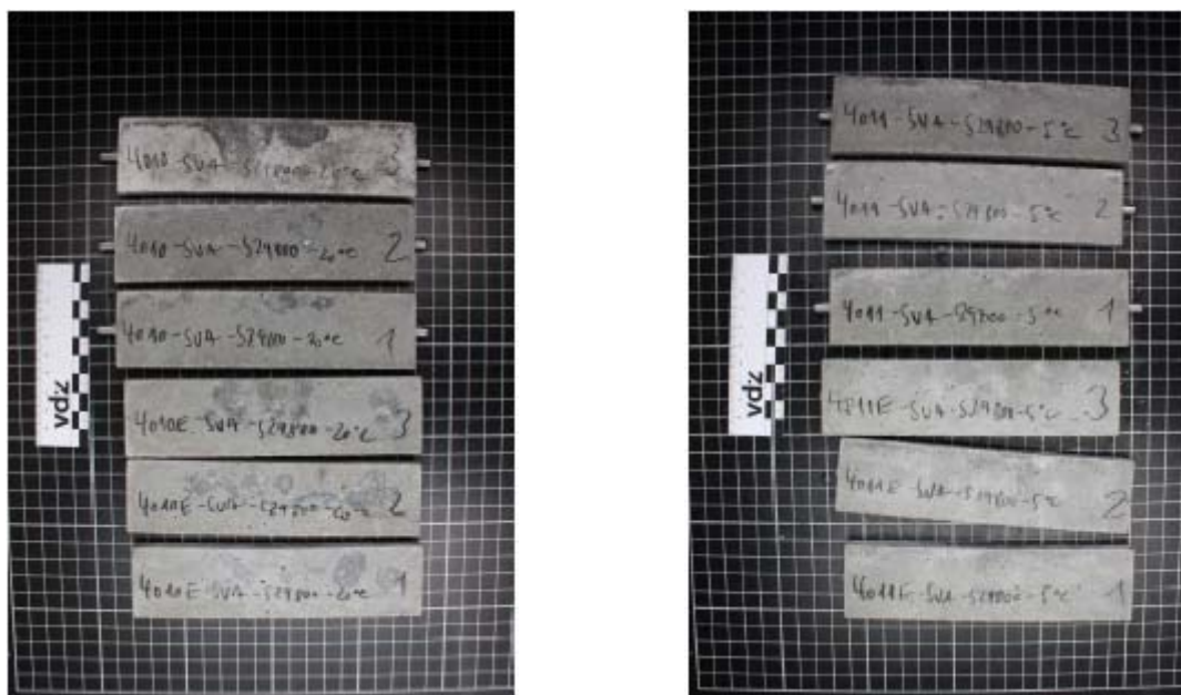
Figure A1: Specimens with CEM III/A XX-LH/SR/LA "Eisenhüttenstadt" after sulfate storage; on the left: after 182 days at 20 °C; on the right: after 91 days at 5 °C
