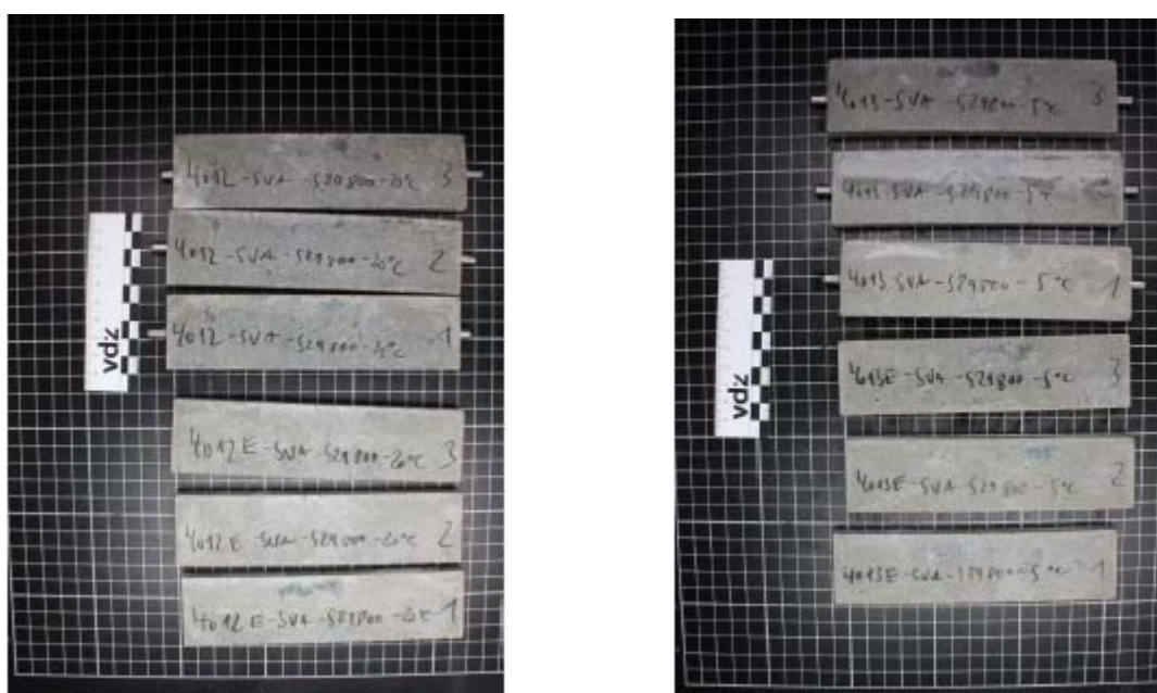
Figure A2: Specimens with CEM III/B 42,5 R-LH/SR after sulfate storage; on the left: after 182 days at 20 °C; on the right: after 91 days at 5 °C
