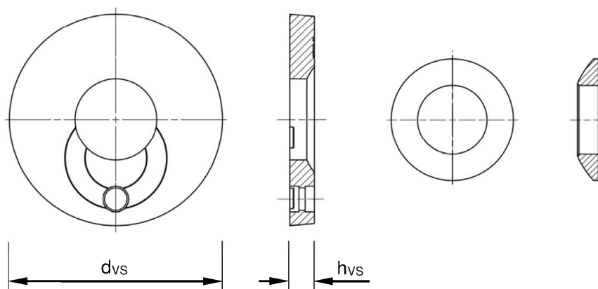
Sealing washer
