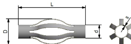
Federkorbdistanzhalter (Maße in mm)
