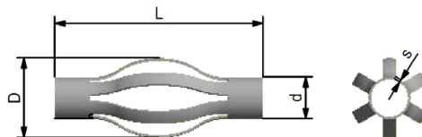
Federkorbdistanzhalter (Maße in mm)
