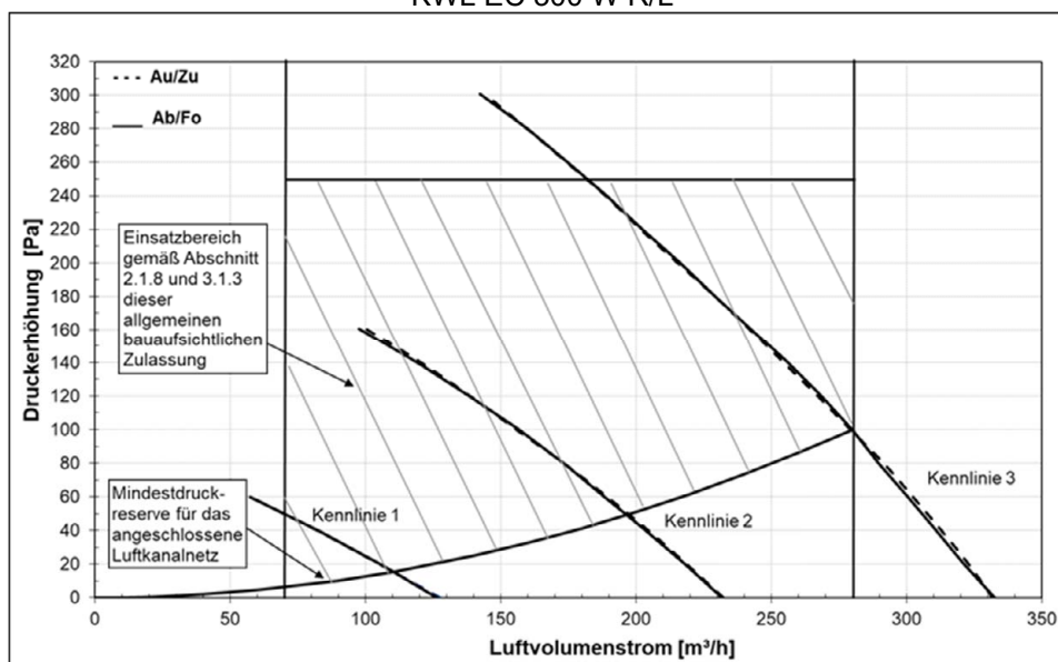
"KWL EC 300 W R/L"
