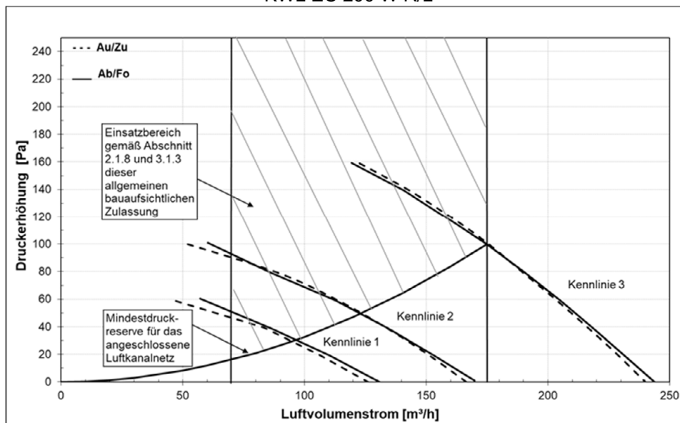
"KWL EC 200 W R/L"
