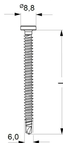
Zahn ZMDS-E 6,0 x L
