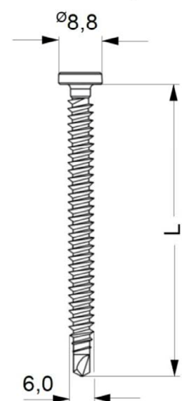
Zahn ZMDS 6,0 x L
