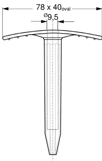
Zahn ZKSH oval
