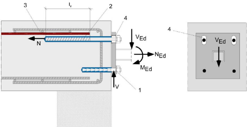
Figure A3.2: Lap of the anchoring of guardrail posts or anchoring of cantilevered building components. In the anchor plate, the drill holes for the fischer rebar anchors have to be designed as slotted holes with axial direction to the shear force.
