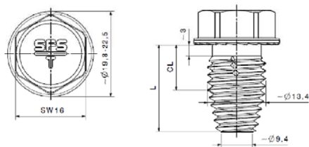
nonut®-TDBL-T-13.4xL nonut®-TDNL-13.4xL
