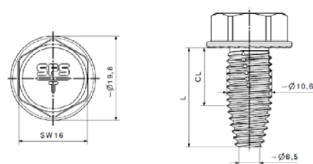
nonut®-TDBLF-T-10.6xL nonut®-TDN-10.6xL
