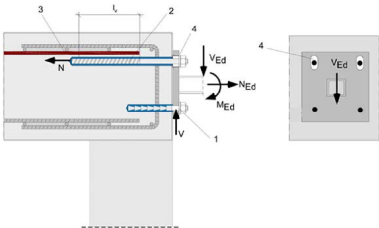
Figure A3.2: Lap of the anchoring of guardrail posts or anchoring of cantilevered building components. In the anchor plate, the drill holes for the Upat rebar anchors have to be designed as slotted holes with axial direction to the shear force.
