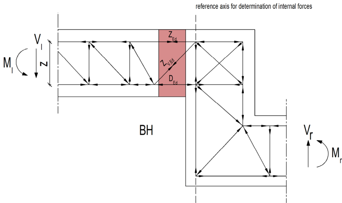
figure D - 7 Egcobox BH – moment and shear force connection with height offset – static system
