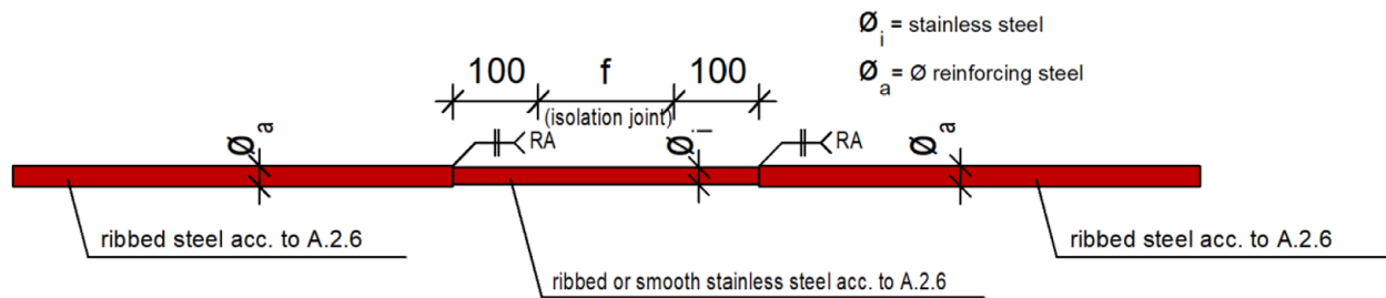
figure A - 31 compression bar version 2 – butt-welded
