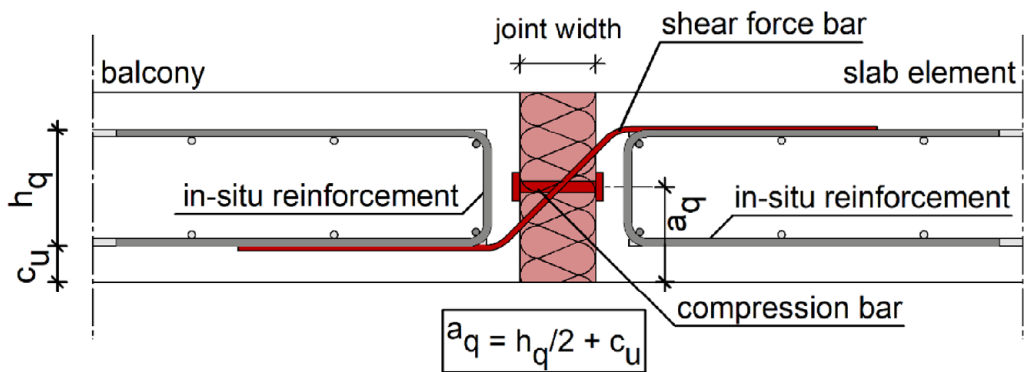
figure A - 6 Egccobox type V – shear force connection with central compression bearing
