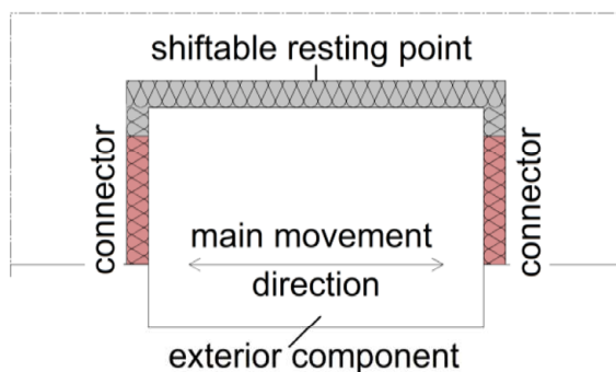
figure B - 2 restraint-free installation for opposing connections
