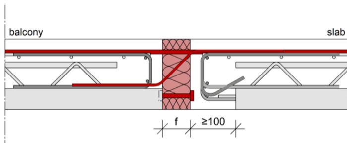
figure B - 7 installation of Egccobox in slab elements – bracket of the shear force bar on the (reflected) element plan and anchor stirrup variations like in B - 4 to B - 6
