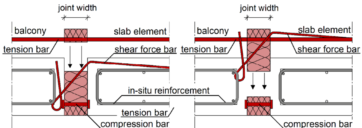
figure A - 2 Egccobox type M – moments and shear force connection for semi-prefab-elements – shear force bar with loop
