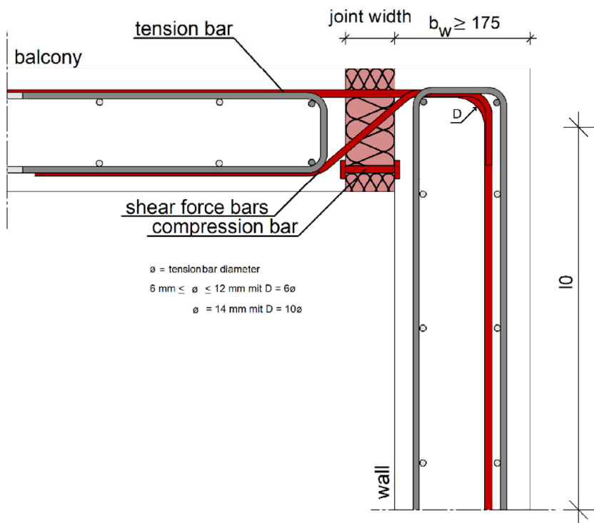
figure A - 19 Egccobox type WU – connection to wall top
