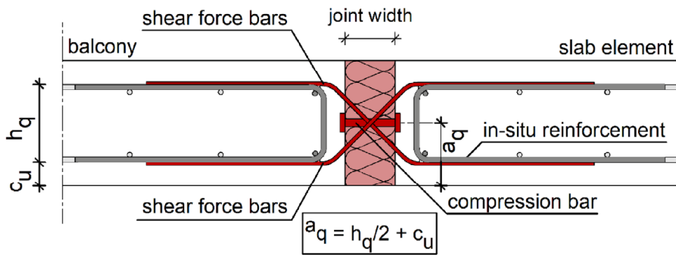
figure A - 8 Egccobox type V± – shear force connection to transfer positive and negative shear forces with central compression bearing
