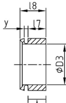
Figure A13: distance sleeve PMB
