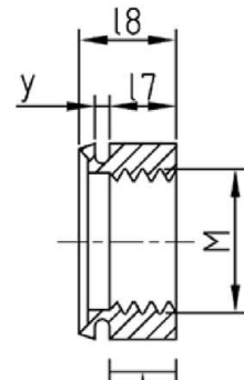
Figure A12: counter nut PMF
