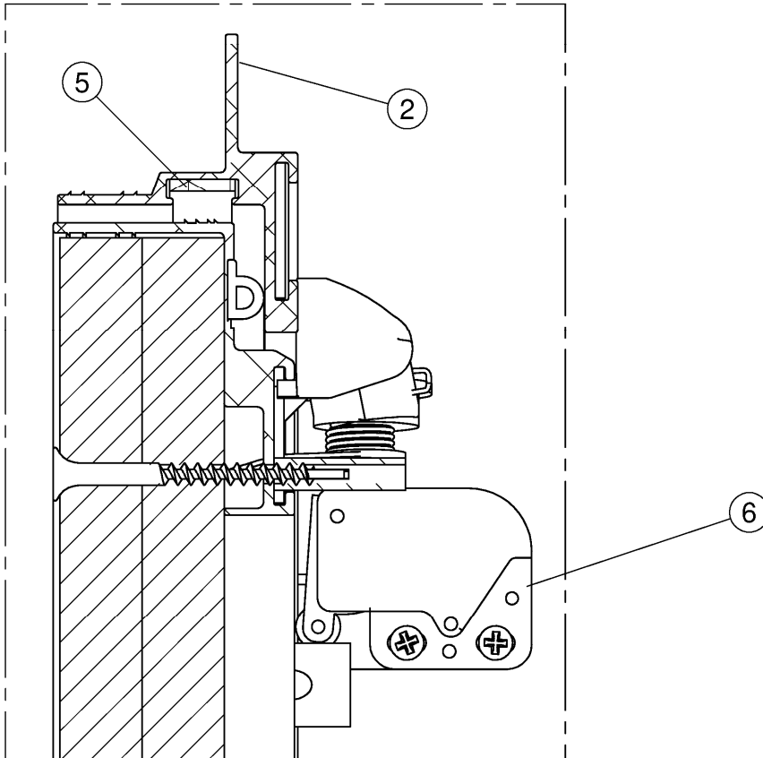
Detail E
