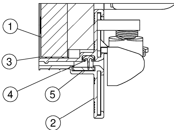
Detail C
