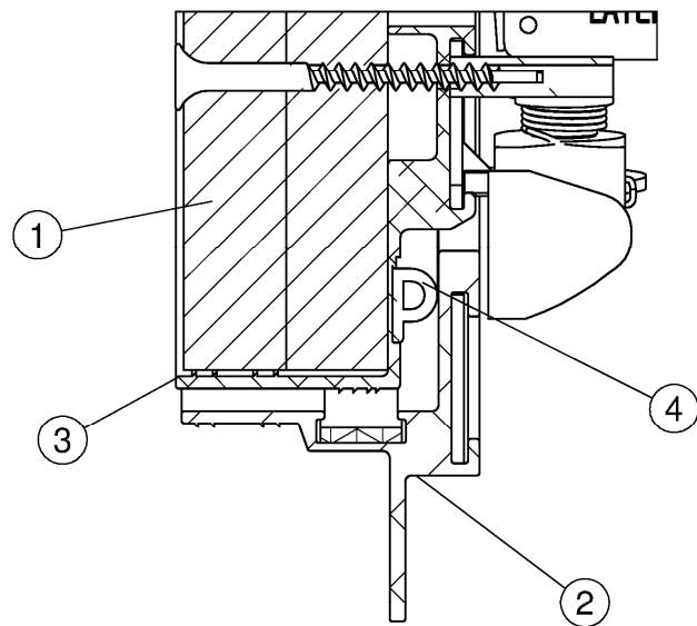
Detail F
