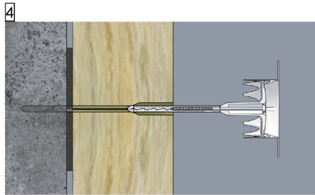
Insert the anchor into the drill hole
