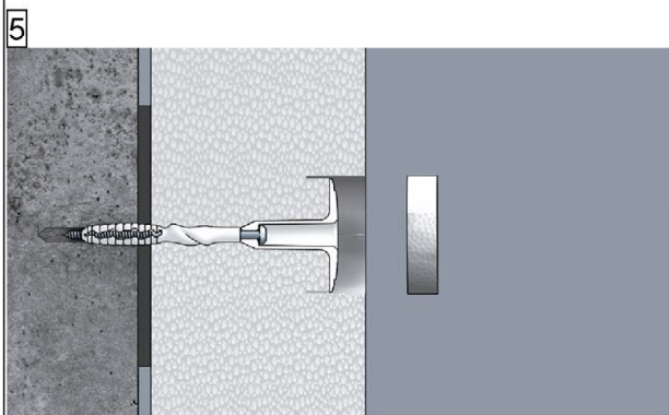
Insert the ejotherm STR - insulation cover with the help of a float
