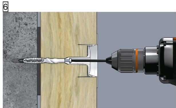
Mounting on the surface with STR tool
