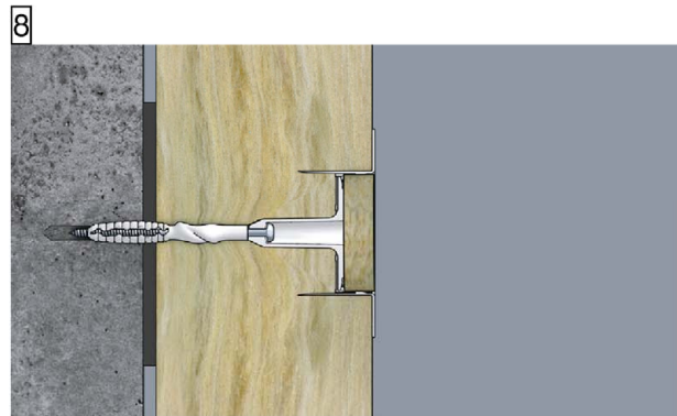
installed anchor
