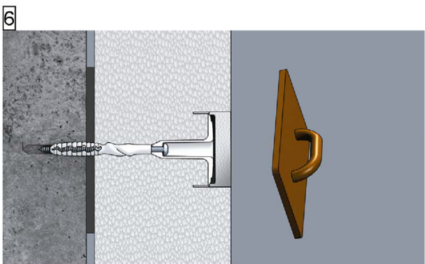
Insert the ejotherm STR - insulation cover with the help of a float
