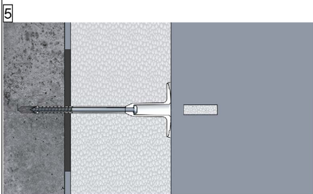
Insert the STR plug
