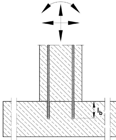
Figure A2: Slab / beam to wall or beam to column
