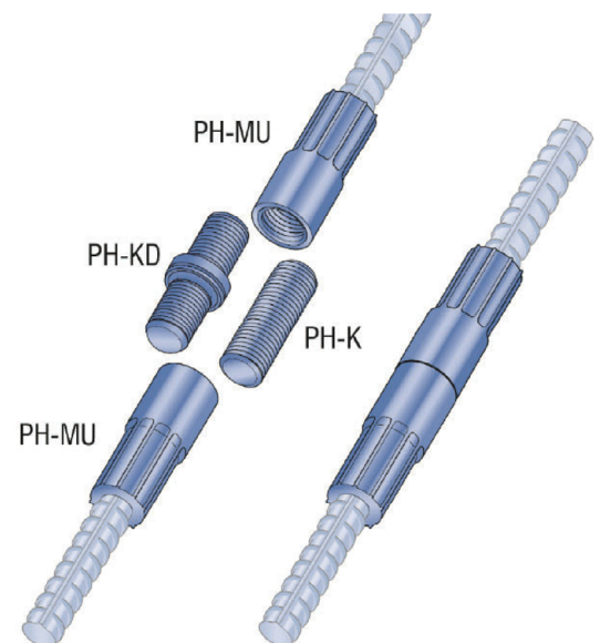
Fig. A2: PH-MU + PH-K / PH-KD + PH-MU
