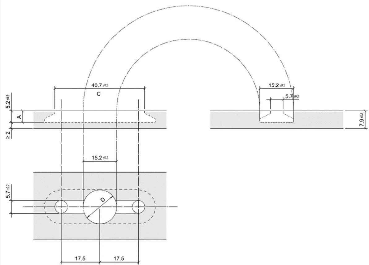
Borehole geometry
