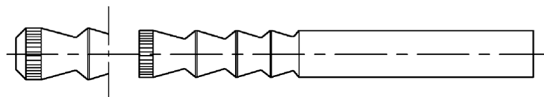
Ankerstange WBAT-IZ
