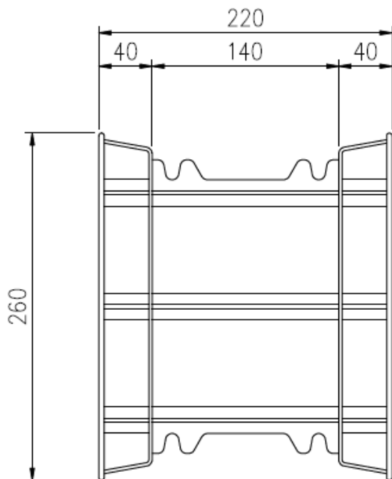
Plastic tie of BEWI main wall PLUS and corner wall block PLUS
