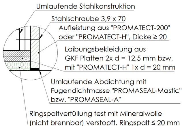
Detail A 1)
