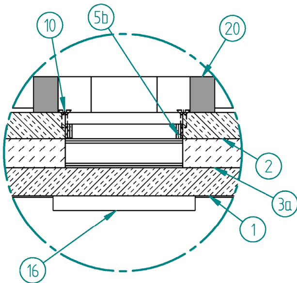
Detail U
