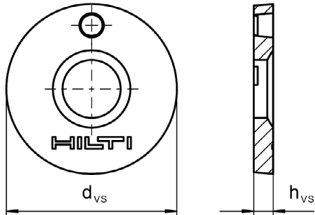
Sealing washer
