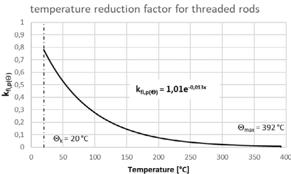
Figure C1 Reduction factor k_{fi,p}(\theta)
