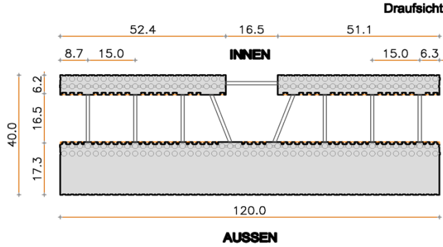
Abmessungen "T"-Element 40/16.5 (120x40x30)
