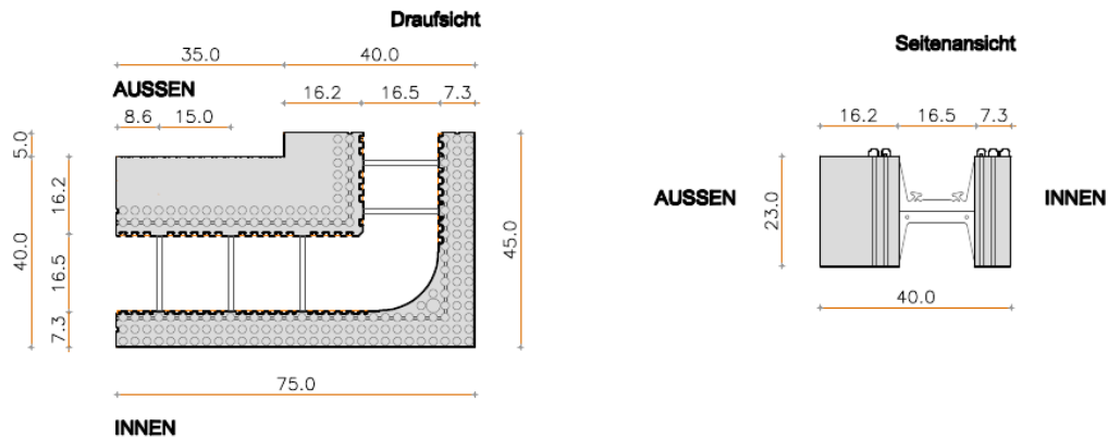
Abmessungen Eckelement Innen 40/16.5 (45-75)x40x23
