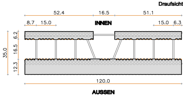
Abmessungen "T"-Element 35/16.5 (120x35x30)
