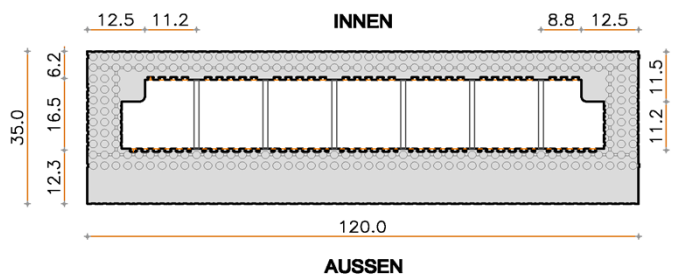
Abmessungen Fenster-Endelement 35/16.5 (120x35x30)
