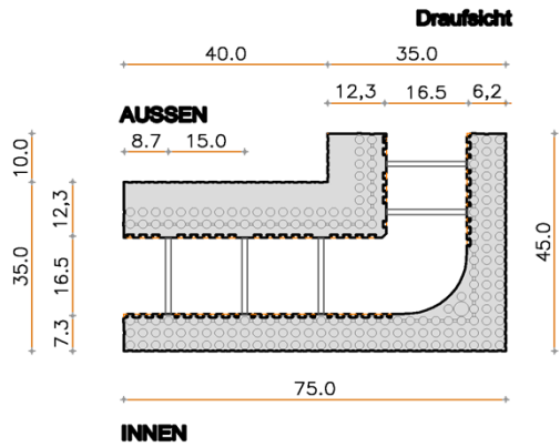
Abmessungen Eckelement Innen 35/16.5 (45-75) 35x30
