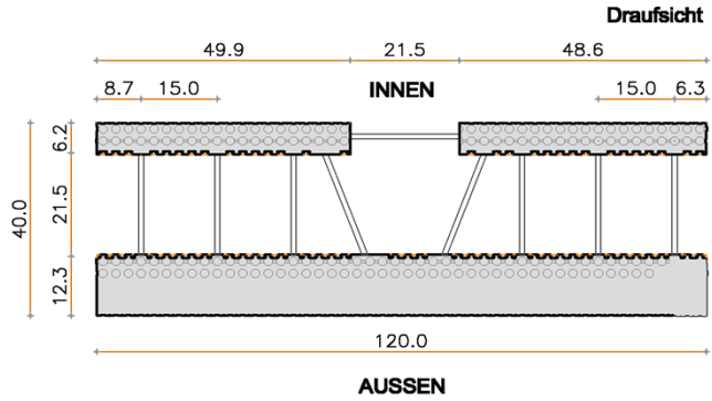
Abmessungen "T"-Element 40/21.5 (120x40x30)
