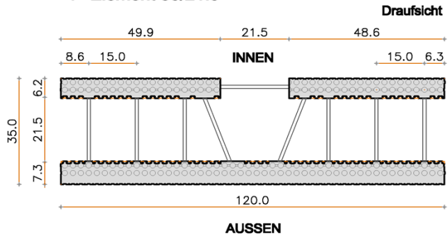
Abmessungen "T"-Element 35/21.5 (120x35x30)
