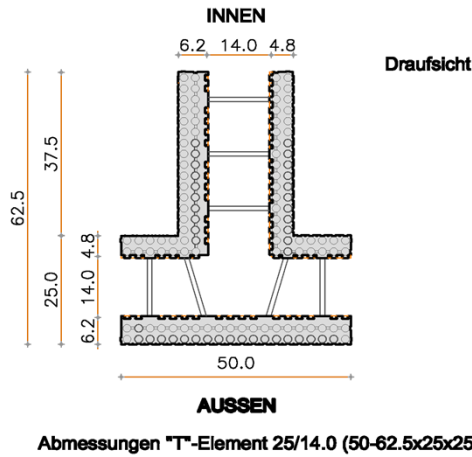
"T"-Element 25/14.0
