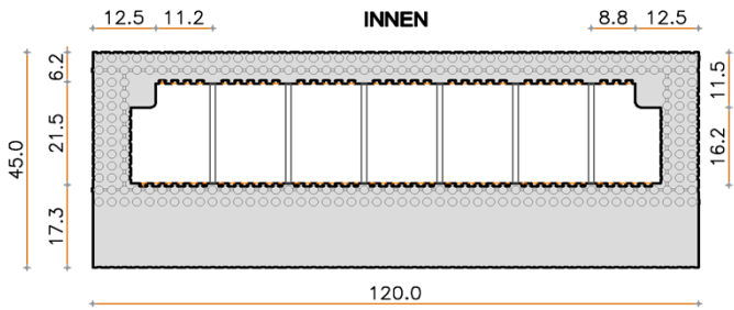
Abmessungen Fenster-Endelement 45/21.5 (120x45x30)
