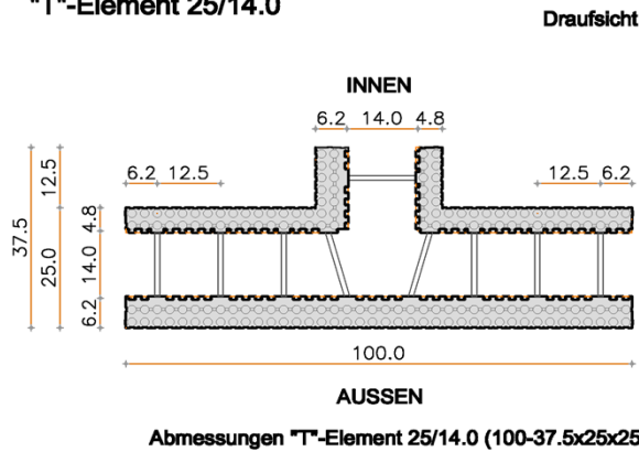
"T"-Element 25/14.0
