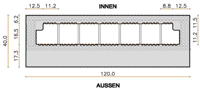
Abmessungen Fenster-Endelement 40/16.5 (120x40x30)
