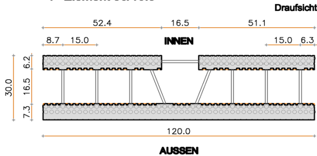
Abmessungen "T"-Element 30/16.5 (120x30x30)
