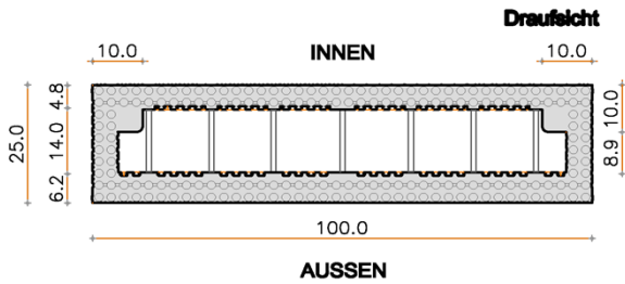
Abmessungen Fenster-Endelement 25/14.0 (100x25x25)
