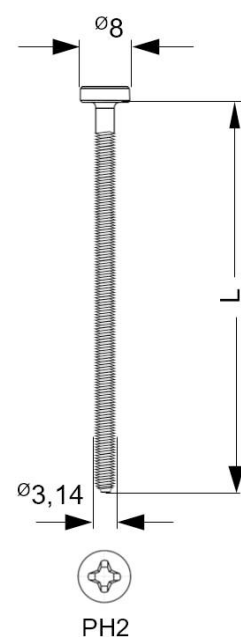
Zahn metric screw-E 3,14 x L
