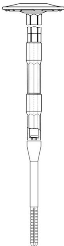
Zahn ZSSB-module-pipe 4,8 with module, dowel attachment and clickplate
