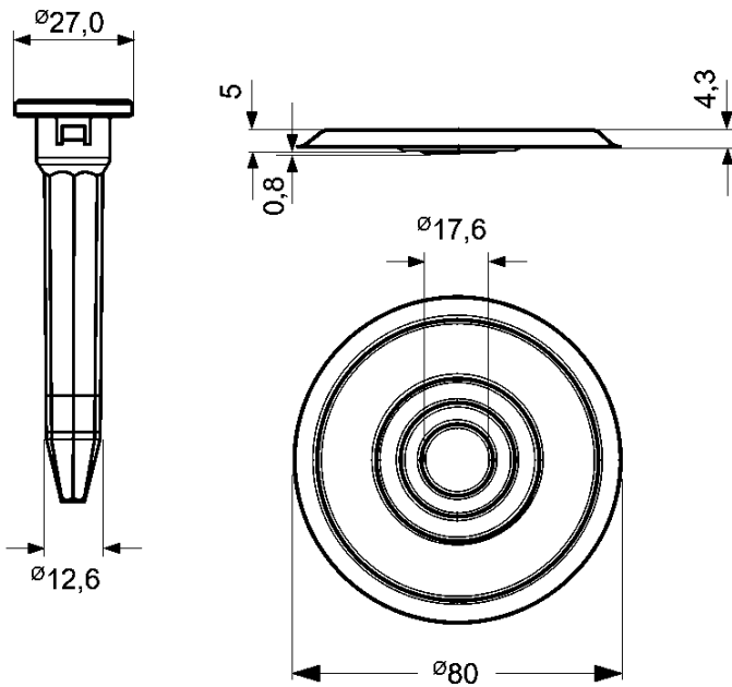
Zahn ZCTS-pipe 4,8 and ZCTS-plate
