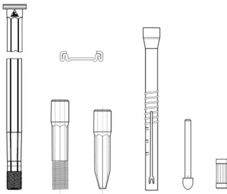
Zahn ZSSB-module-pipe 4,8 with module, expanding dowel attachment and bar
