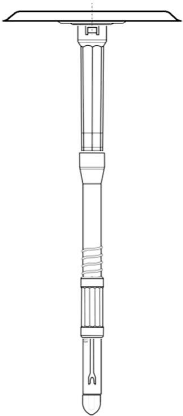
Zahn ZCTS-pipe 4,8 with ZCTS-plate with expanding dowel attachment
