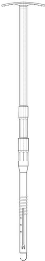
Zahn ZKSH oval module 4,8 with expanding dowel attachment
