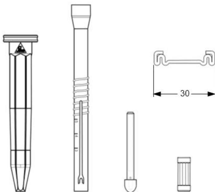
Zahn ZSSB-pipe 4,8 with expanding dowel attachment and bar
