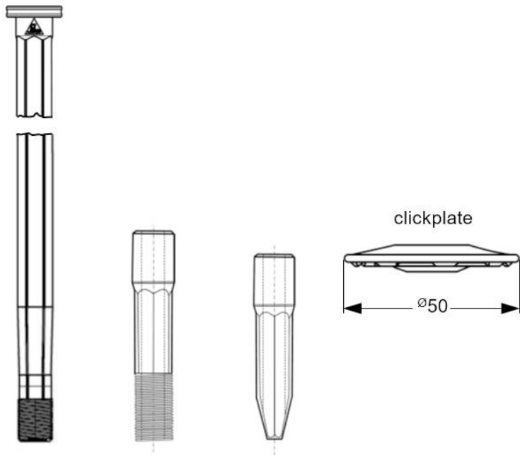
Zahn ZSSB-module-pipe 6,0 with module and clickplate
