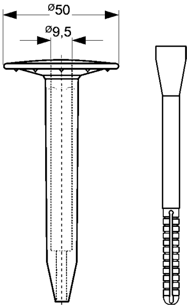
Zahn ZKSH round with dowel attachment
