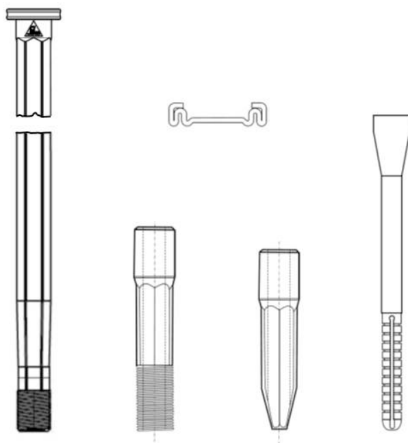
Zahn ZSSB-module-pipe 4,8 with module, dowel attachment and bar
