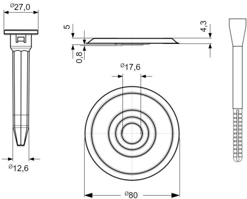
Zahn ZCTS-pipe 4,8 with ZCTS-plate and dowel attachment
