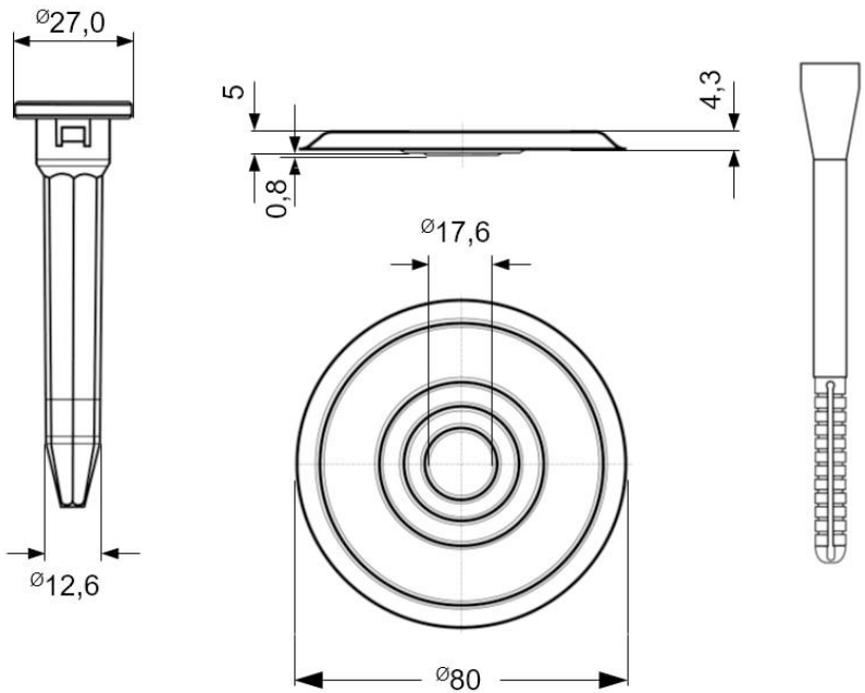
Zahn ZCTS-pipe 4,8 with ZCTS-plate and dowel attachment
