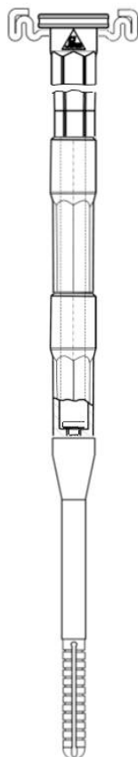
Zahn ZSSB-module-pipe 4,8 with module, dowel attachment and bar
