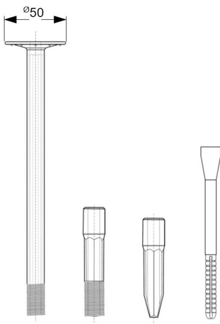
Zahn ZKSH round module 4,8 with dowel attachment
