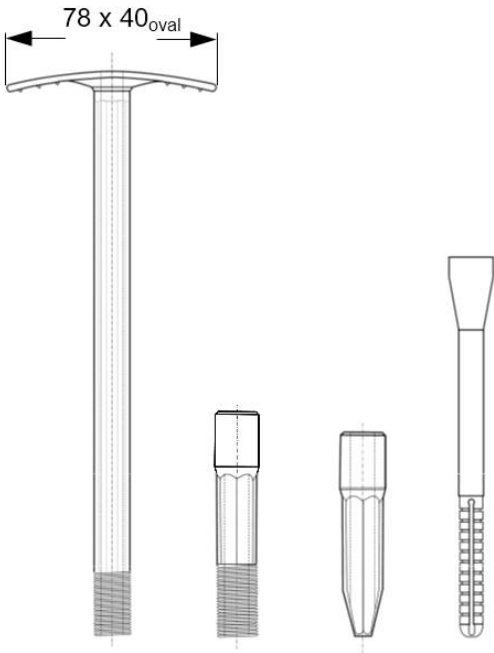
Zahn ZKSH oval module 4,8 with dowel attachment
