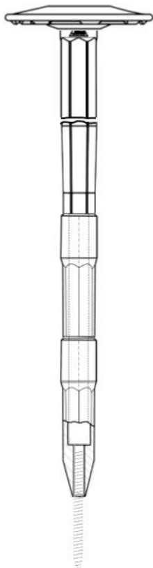
Zahn ZSSB-module-pipe 4,8 with module and clickplate
