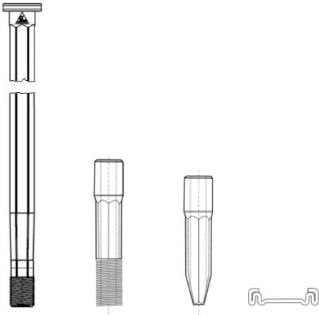
Zahn ZSSB-module-pipe with module 6,0 and bar
