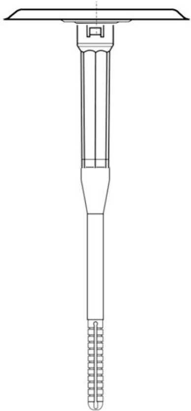
Zahn ZCTS-pipe 4,8 with ZCTS-plate and dowel attachment
