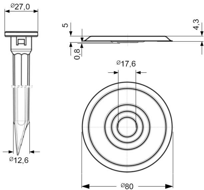
Zahn ZCTSplus-pipe 4,8 and ZCTS-plate
