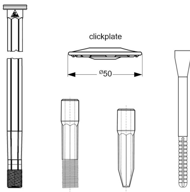
Zahn ZSSB-module-pipe 4,8 with module, dowel attachment and clickplate
