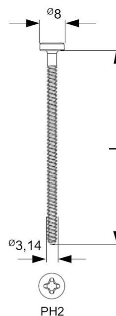
Zahn metric screw-E 3,14 x L
