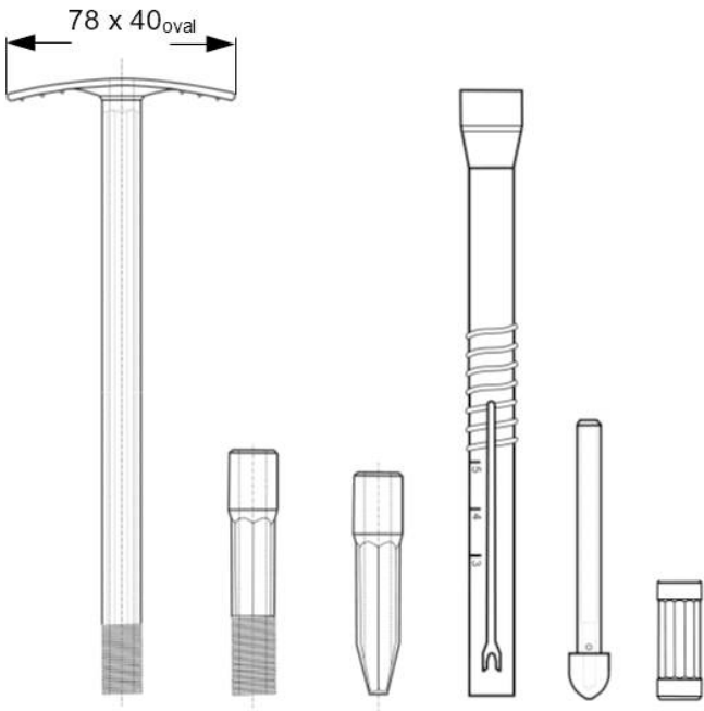
Zahn ZKSH oval module 4,8 with expanding dowel attachment
