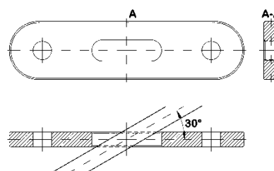
Cross plate 30°
