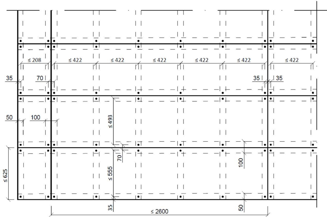
cladding with 20mm thick fire protective boards
