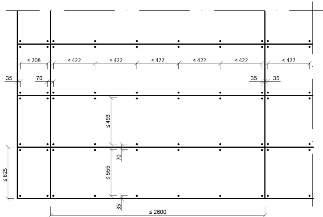
cladding with 20mm thick fire protective boards
