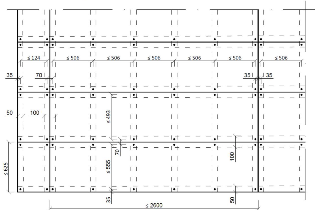
cladding with 30mm thick fire protective boards
