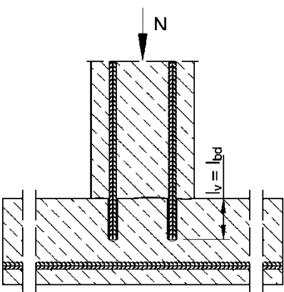
Figure A4: Rebar connection for components stressed primarily in compression.
