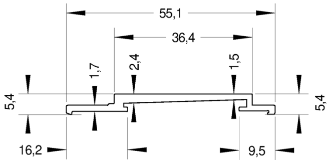
Additional profil F67
