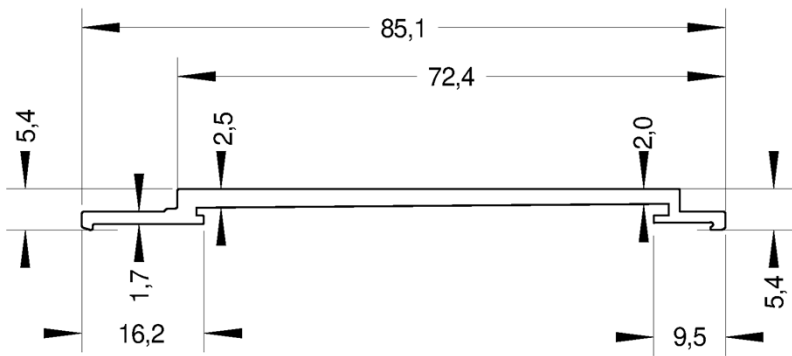
Additional profil F68
