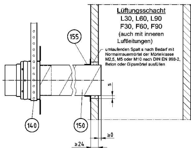
Detail X
