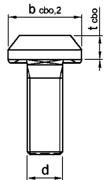
Double notching channel bolts JKB, JKC
