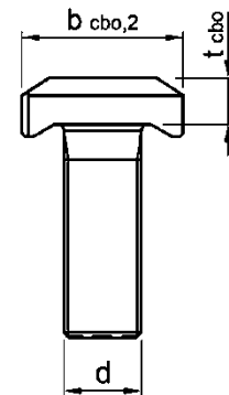
Hooked channel bolts JA, JB, JC
