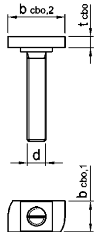
Hammerhead channel bolts JD, JH
