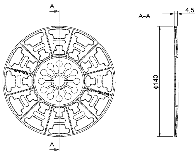
TDX-P-140/TDX-140
