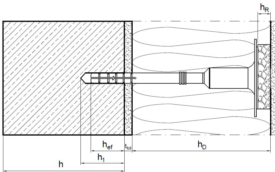
immersed mount
