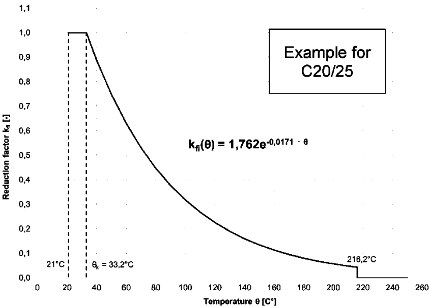
Figure C1 Example graph of reduction factor k_{fi}(\theta) = k_{fi,100y}(\theta) for concrete strength class C20/25 for good bond conditions:
