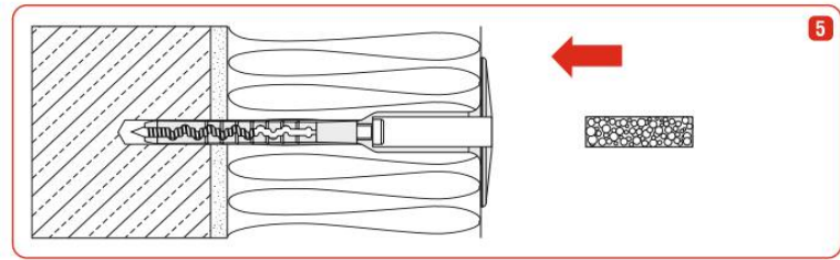
Fig. 5 Insert the KSV to be flush with the plate surface.
