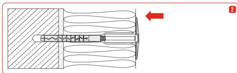
Fig.2 Place the anchor into the drill hole. The bottom side of the plate must be flush with the thermal insulation surface.
