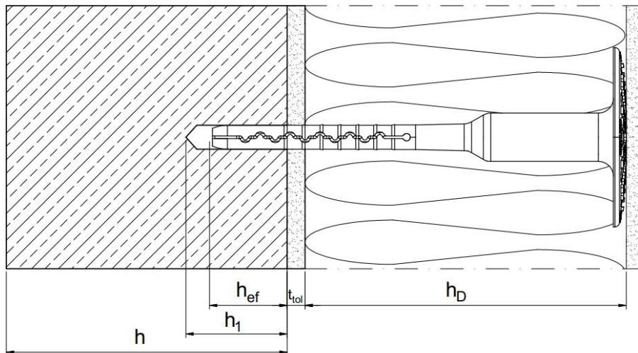
surface mount
