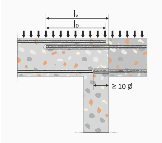
Figure A3: End anchoring of slabs or beams (e.g. designed as simply supported)
