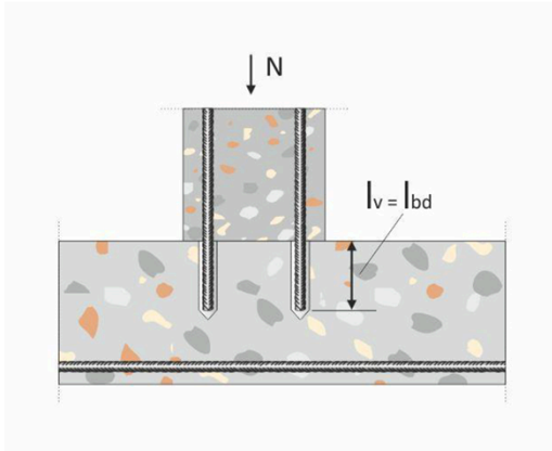
Figure A4: Rebar connection for components stressed primarily in compression. The rebars are stressed in compression
