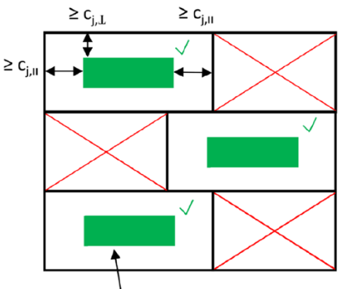
Single anchor
