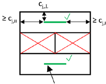
Single anchor
