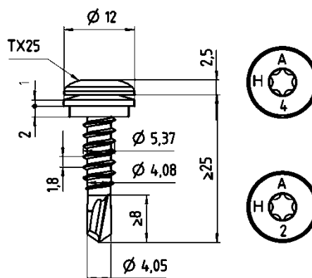
Hilti S-AD 31 LPS 5,5xL * (Typ I2) Hilti S-AD 31 LPSS 5,5xL ** (Typ I2)
