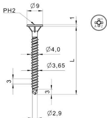
Hilti S-PD 01 S 4,0xL * (Typ J)
