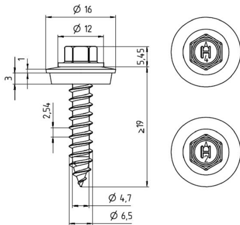
Hilti S-MP 53 S 6,5xL * (Typ L2) Hilti S-MP 53 SS 6,5xL ** (Typ L2)
