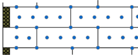
12 (8/4) Dübel/m 2
