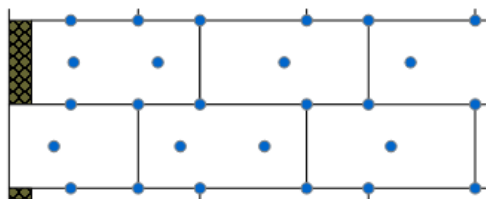
7 (3/4) Dübel/m 2
