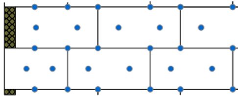
8 (4/4) Dübel/m 2
