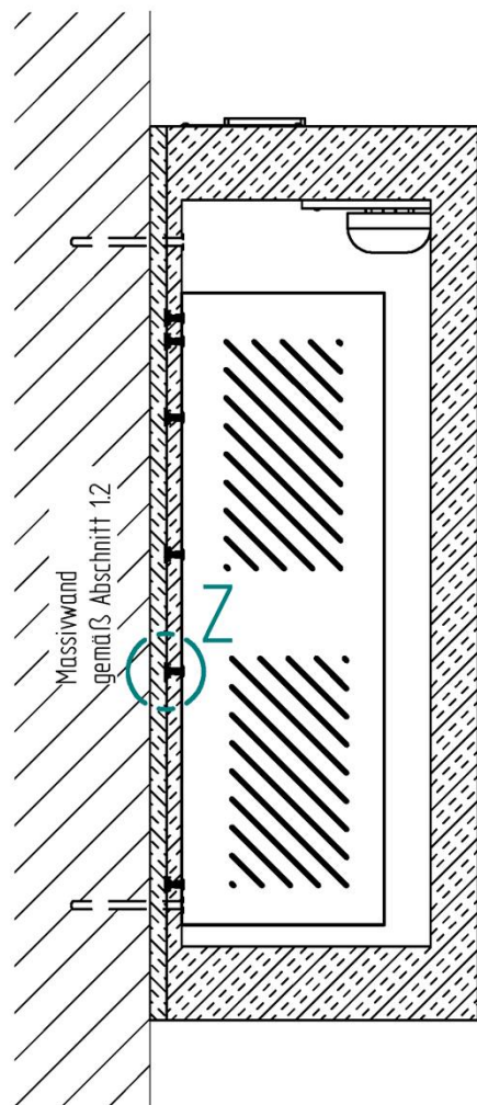
Detail Z
